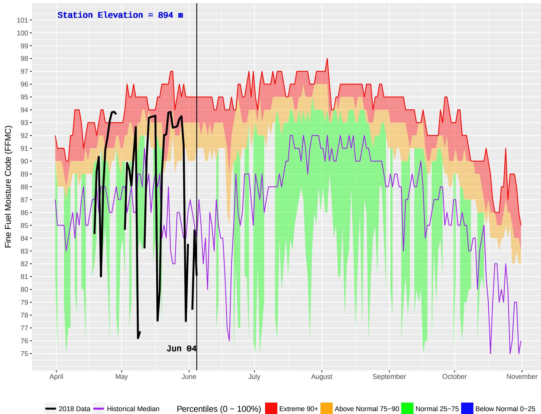
TOBY HUB (417) : Historical (1986–2016) and Current (2018) Noon Fine Fuel Moisture Code (FFMC)
