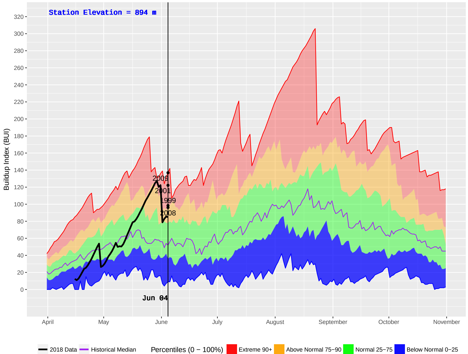
TOBY HUB (417) : Historical (1986–2016) and Current (2018) Noon Buildup Index (BUI)
