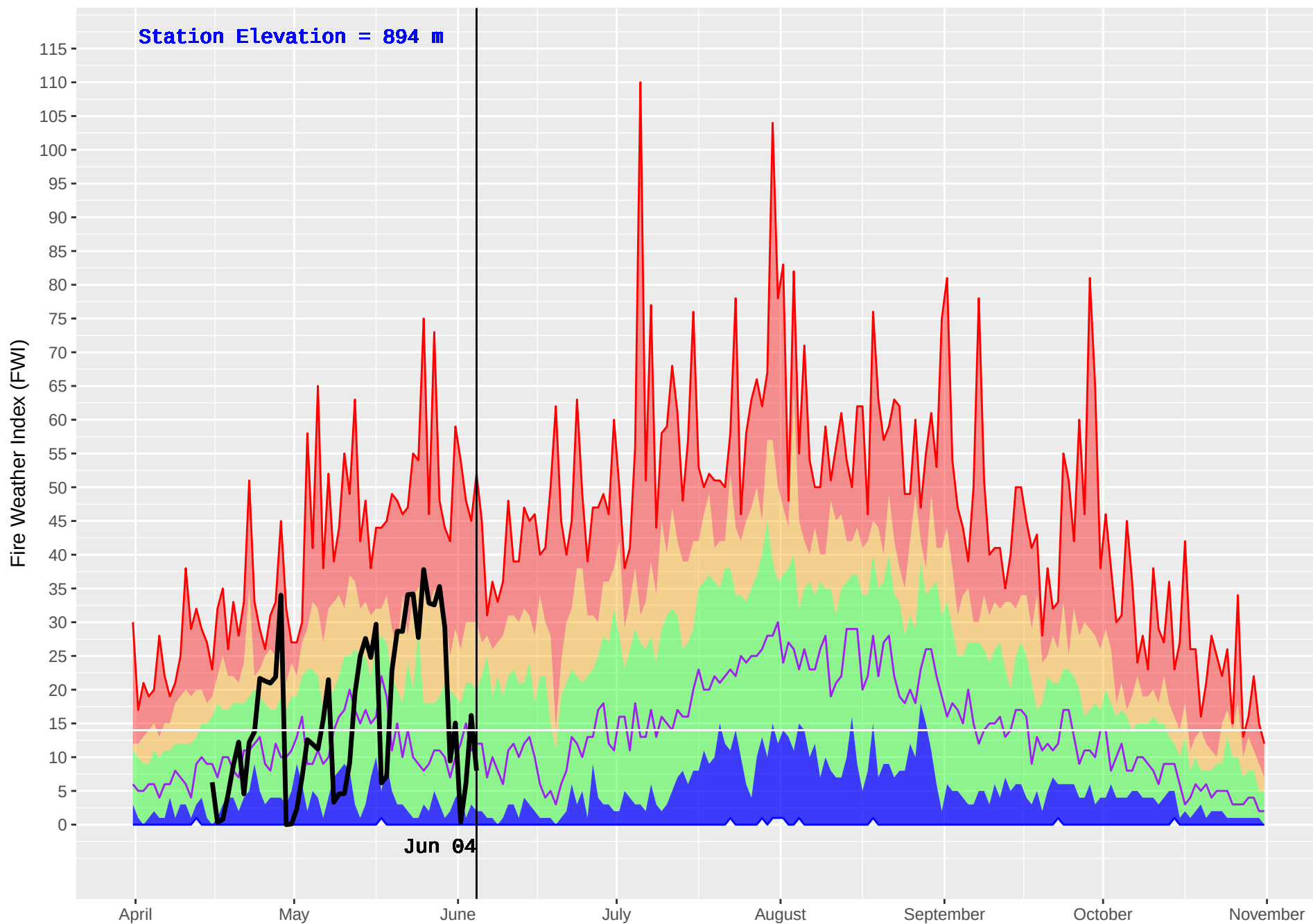
TOBY HUB (417) : Historical (1986–2016) and Current (2018) Noon Fire Weather Index (FWI)
